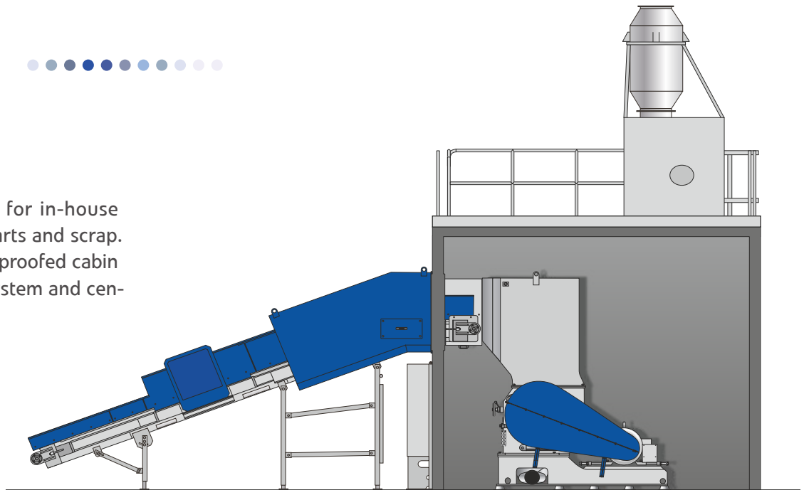
Two stage size reduction system consisting of ZERMA single shaft shredder and GSE granulator.
